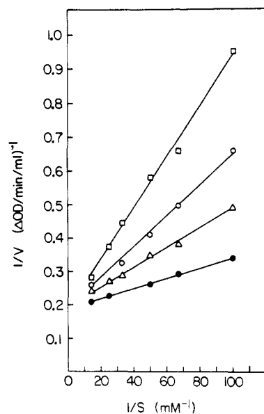
Figure 2. Inhibition of parasite lactate dehydrogenase by gossylic nitrile 1,1'-dibutyrate. Initial rates were determined in the absence of drug (●) or in the presence of 0.625 \mu\text{M} ( \Delta ), 1.25 \mu\text{M} (○), or 2.50 \mu\text{M} (□) drug. NADH is the varied substrate, S. Inhibition is competitive, K_i = (6.2 \pm 0.2) \times 10^{-7} M.
