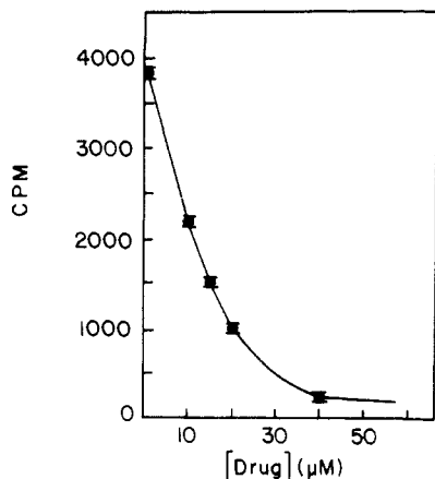
Figure 1. Inhibition of growth of P. falciparum , strain CDC/I/HB-3, by gossylic nitrile 1,1'-divalerate, as determined by uptake of [ ^3\text{H} ]hypoxanthine: \text{LD}_{50} = 12 \mu\text{M} .
